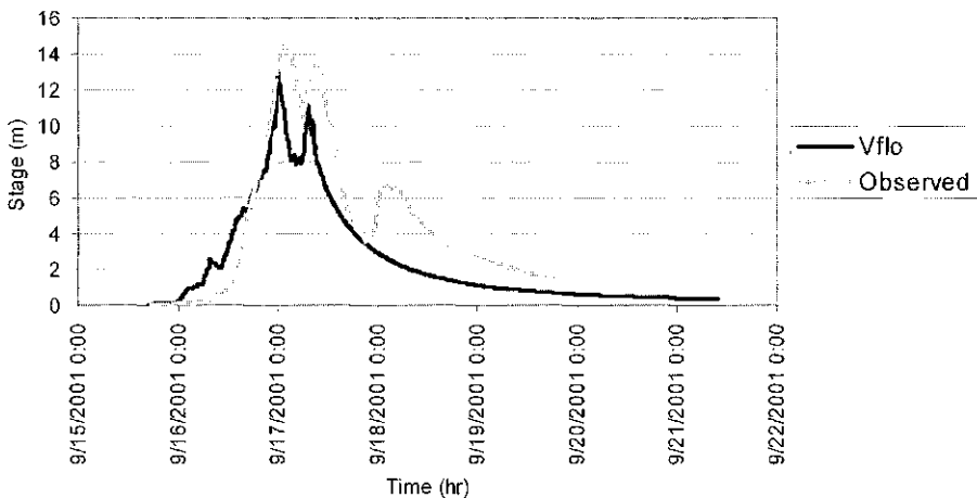
Fig. 4 Simulated and observed stage hydrographs at the Wu Du Bridge.
