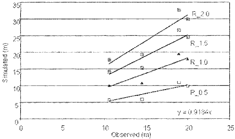
Fig. 3 Stage sensitivity to radar rainfall scalars.
