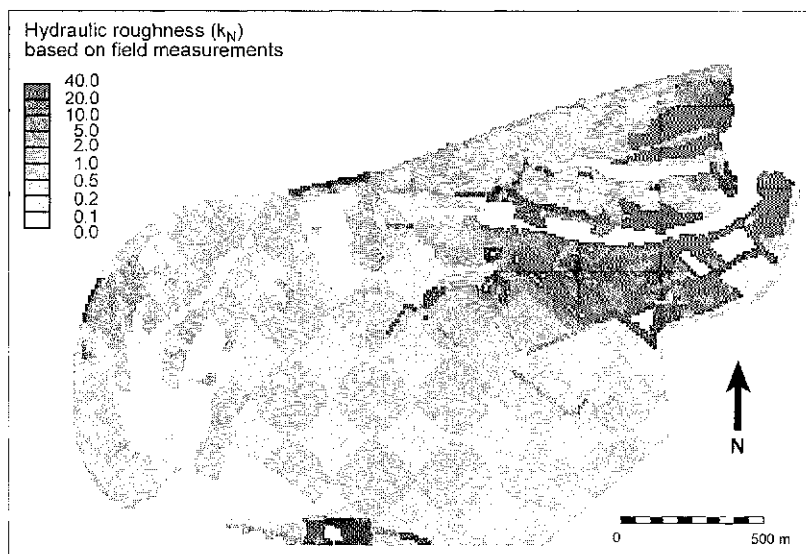
Fig. 5 Map of the hydraulic roughness of vegetation based on field measurements.
