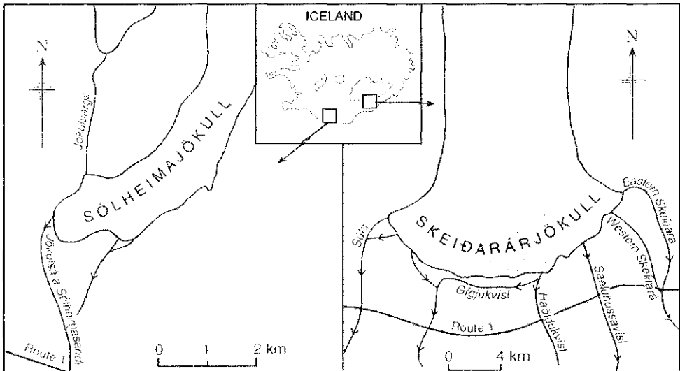
Fig. 1 Location of Sólheimajökull and Skeiðarárjökull, Iceland.
