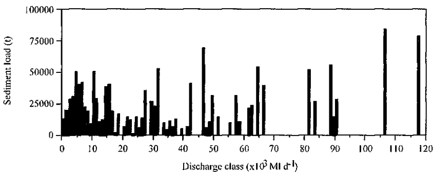
Fig. 4 Magnitude vs frequency histogram for the Richmond River upstream from Casino.
