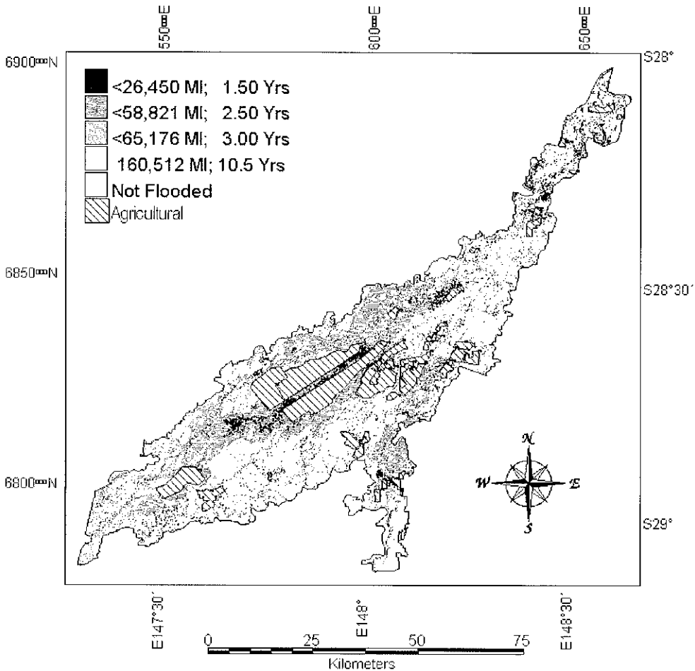
Fig. 2 Flood plain inundation in the lower Balonne. Flood frequency classes are shown as the Q p14 discharge for each inundation area and the average recurrence interval of flooding. ARI zones have been grouped for display purposes.
