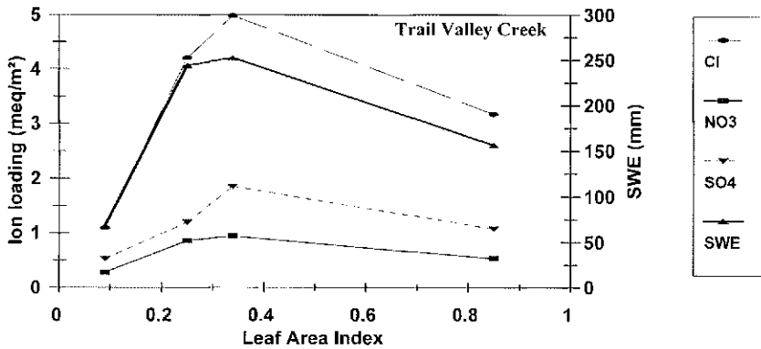
Fig. 1 Ion load and snow water equivalent as functions of leaf area index in transitional spruce forest, shrub tundra and sparse tundra for Trail Valley Creek, near Inuvik, Northwest Territories, Canada.
