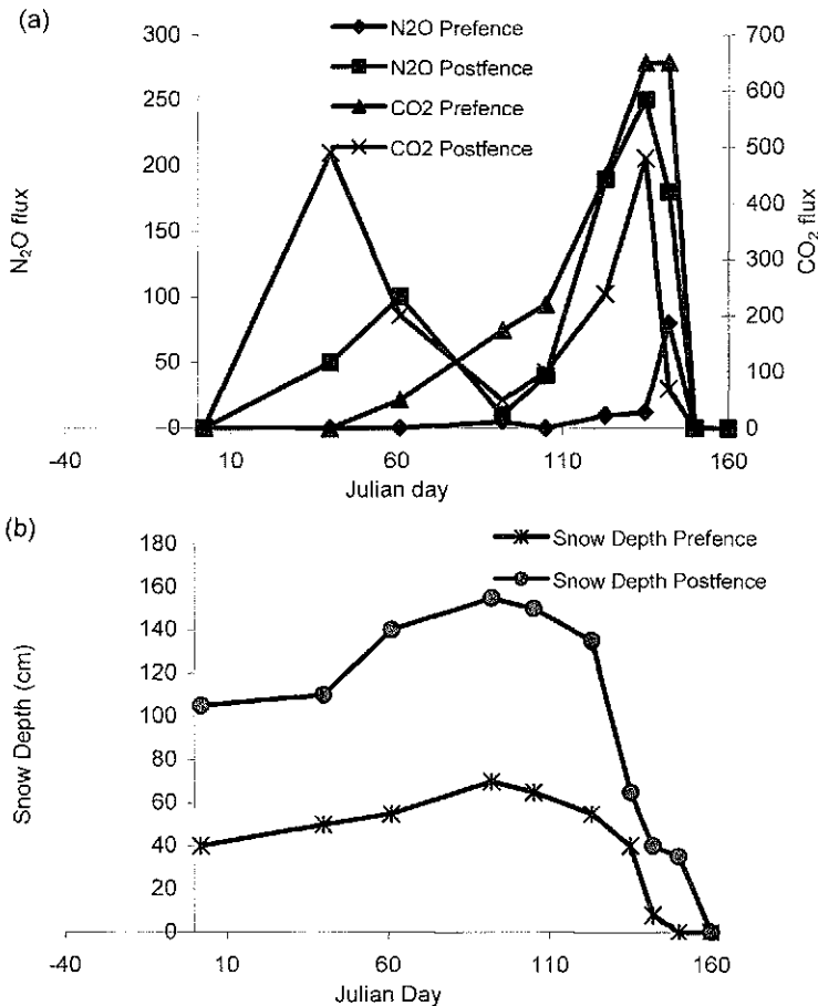
Fig. 2 Subnival \text{CO}_2 and \text{N}_2\text{O} fluxes as a function of snow depth before (1993, n = 6 ) and after (1994, n = 9 ) installation of a snow fence, Rocky Mountains, Colorado, USA.
