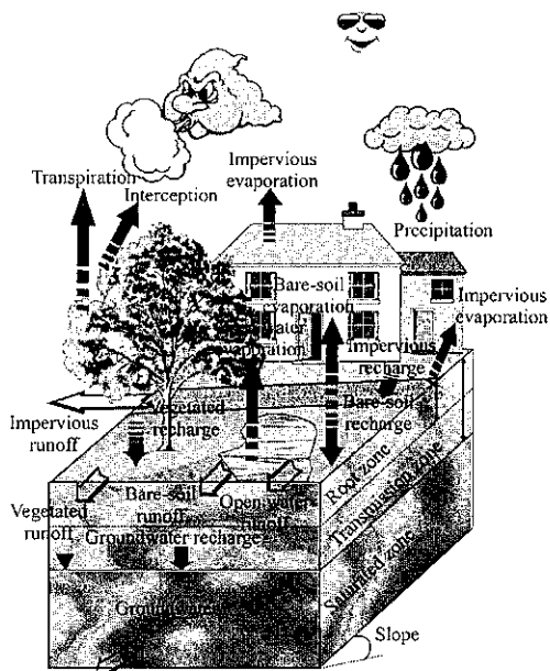
Fig. 1 Schematic water balance of a hypothetical raster cell.
