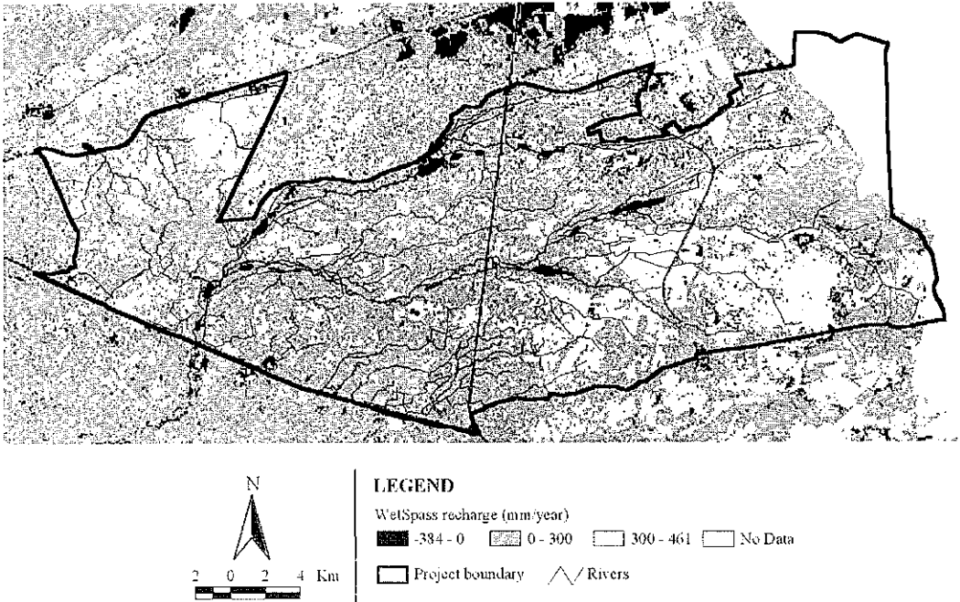
Fig. 4 WetSpss calculated recharge for the Grote Nete area.
