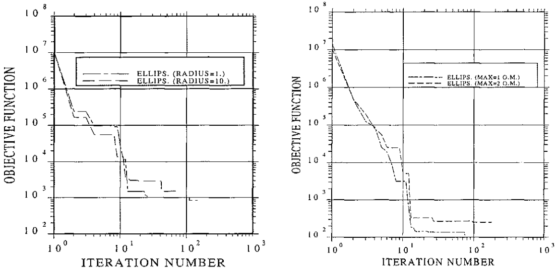
Fig. 3 Sensitivity of the hybrid method to the initial search radius, using the ellipsoids perturbation scheme (left), and to the limits on the size of parameter change per iteration (OM denotes order of magnitude).
