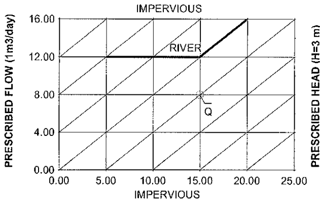
Fig. 1 Flow domain and boundary conditions.
