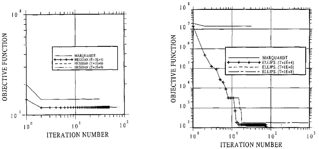
Fig. 2 Comparison between Marquardt's and the hybrid method using (left) Hessian matrix and (right) ellipsoids perturbation schemes, for three initial temperatures.
