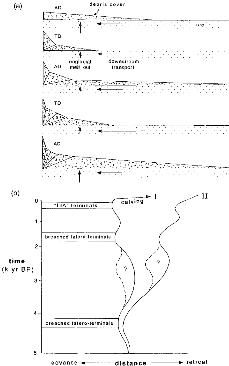
Fig. 2 Schematic evolution of a debris-cover tongue over multiple mass-balance cycles, showing net debris accumulation and glacier expansion.
