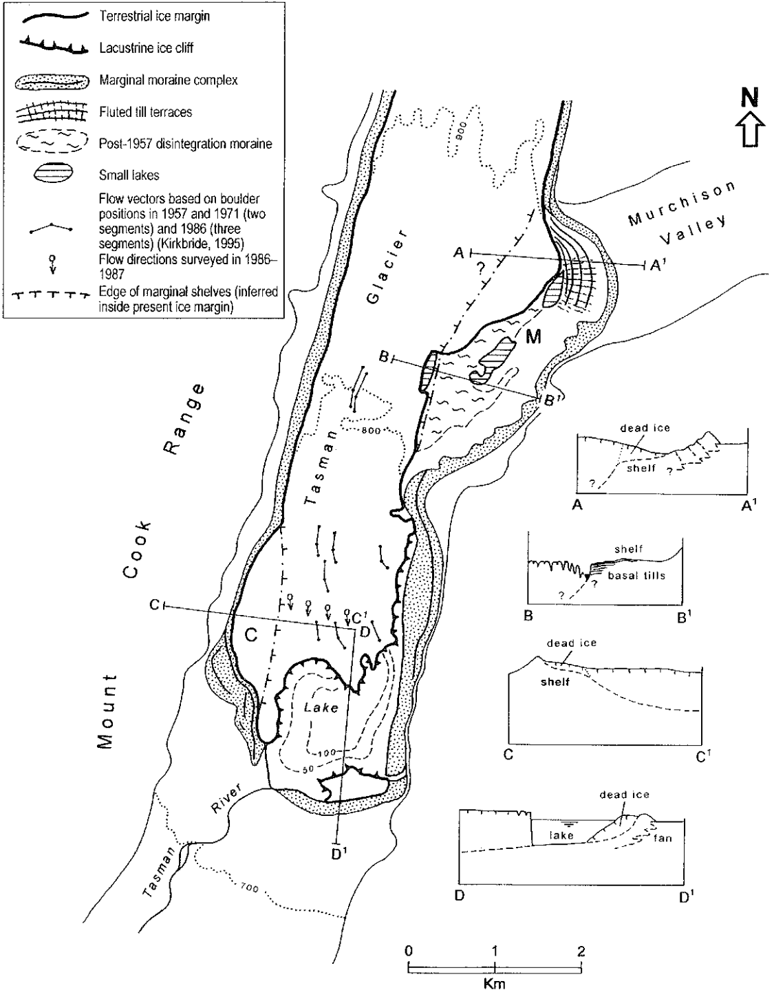
Fig. 1 Map showing the spatial relationships between the present Tasman Glacier and ice-marginal sediment-landform associations, compiled from various sources (see text). Lake bathymetry from Hochstein et al. (1995). Inset sections based on 1:50 000 NZMS 260 topomap, with 2.5× vertical exaggeration.
