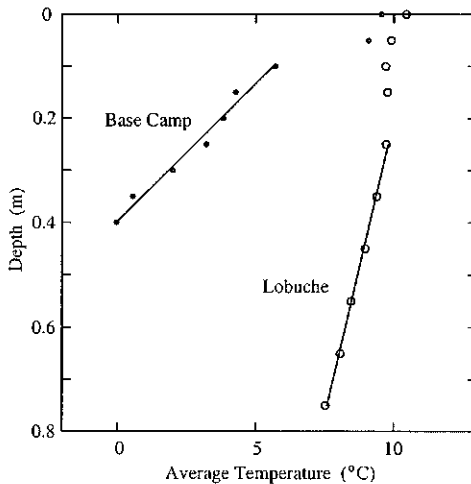
Fig. 4 Average temperature profiles at Base Camp and Lobuche.
