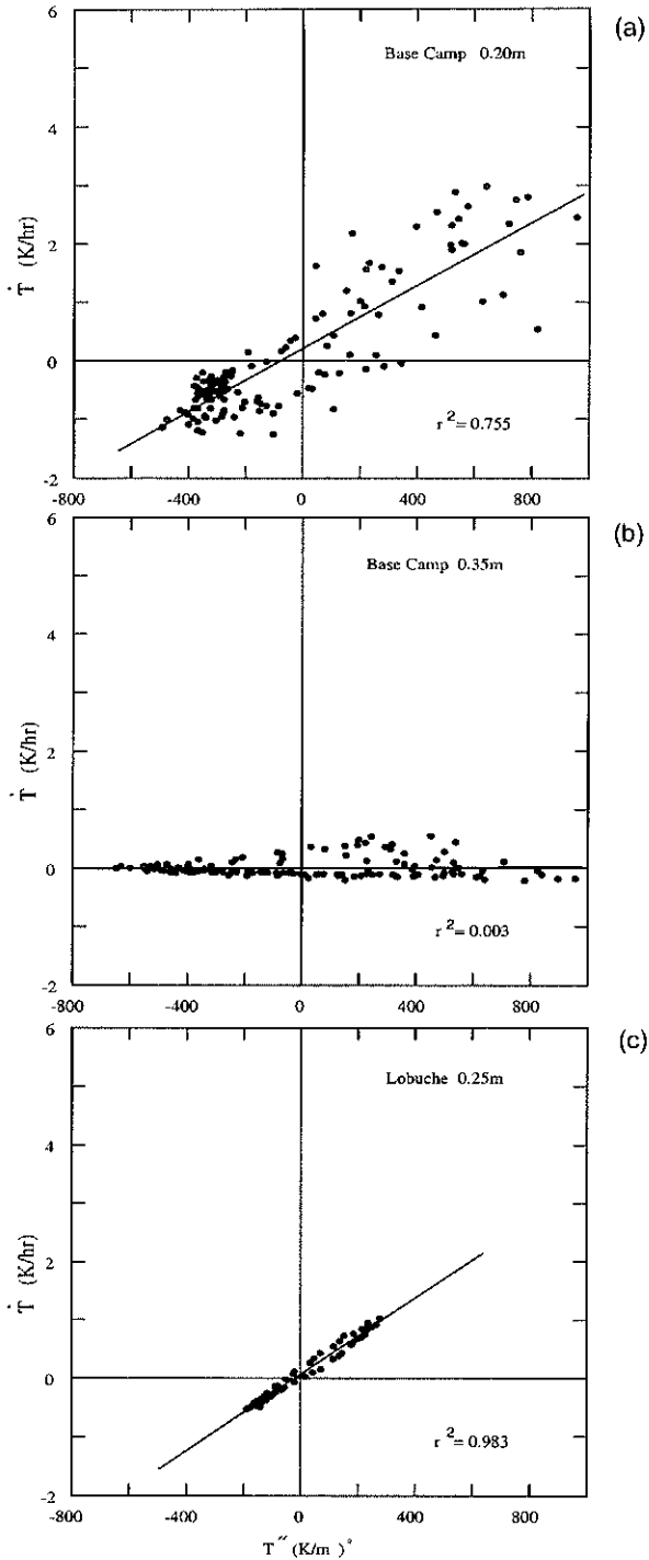
Fig. 5 Distributions of \dot{T} vs T'' at selected depths within the supraglacial debris at study sites near Base Camp ((a) and (b)), and Lobuche (c). The slope of the best fitting line gives an estimate of \kappa (equation (2)).
