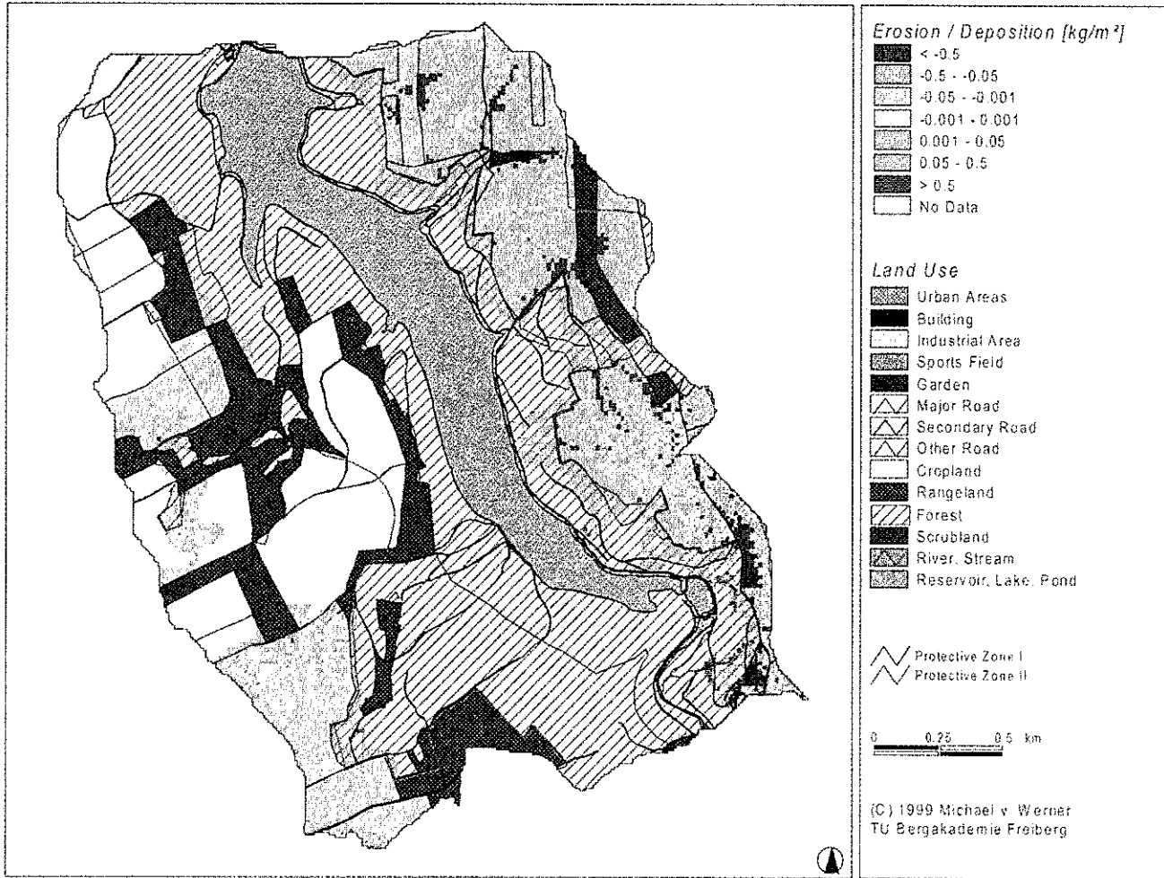
Fig. 1 Erosion map for a sub-watershed of the Klingenberg-Lehnmühle watershed (predicted for the rainfall event on 7 July of the reference-year rainfall scenario; Schmidt & von Werner, 1998).
