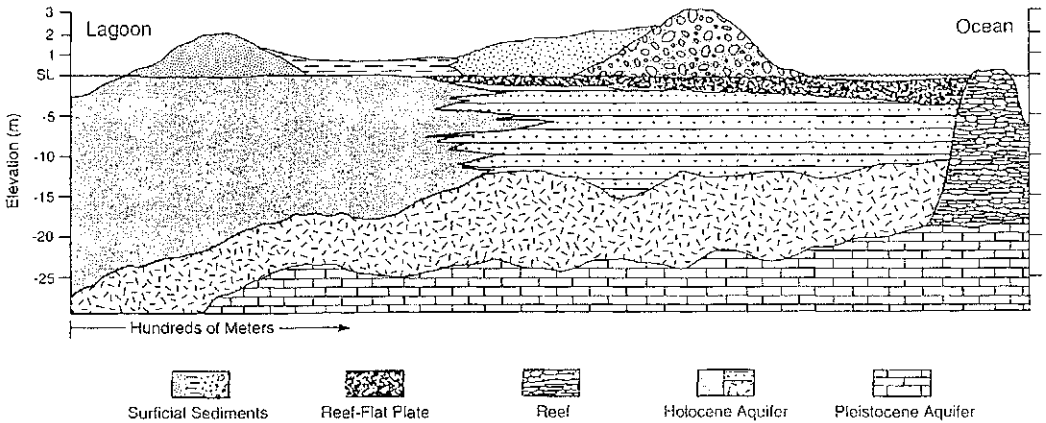
Fig. 1 Schematic diagram of the geological composition of a typical atoll platform.
