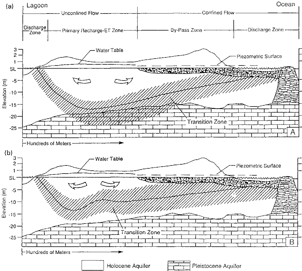
Fig. 3 Groundwater flow patterns for recharge and evapotranspiration conditions prevalent (a) during the wet season and (b) during the dry season.
