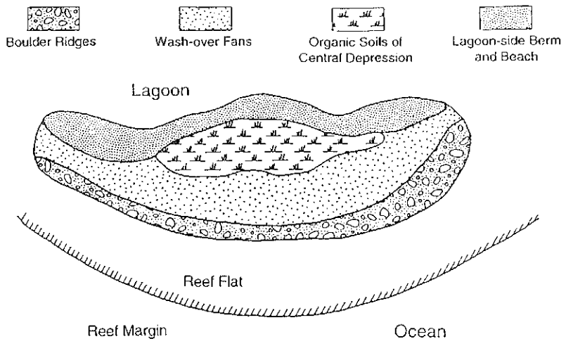
Fig. 2 Areal distribution of general physiographic features for a typical atoll island.
